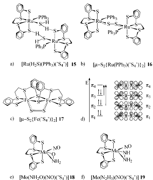
FIGURE 5. Molecular structures of \text{H}_2\text{S} and \mu\text{-S}_2 complexes (a, b, and c), the 4c-6e \pi system of the [\text{M}-\text{S}=\text{S}-\text{M}] cores (d), and the \eta^2 side-on binding of \text{NH}_2\text{O} and \text{N}_2\text{H}_3 to [\text{MS}] cores (e and f).
