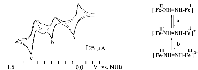
FIGURE 8. Cyclic voltammogram of [\mu\text{-N}_2\text{H}_2\{\text{Fe}(\text{PPR}_3)(\text{S}_4')\}_2] ( 25 ) (in \text{CH}_2\text{Cl}_2 , 20^\circ\text{C} , v = 100\text{ mV/s} ) and assignment of redox waves and Fe oxidation states.
