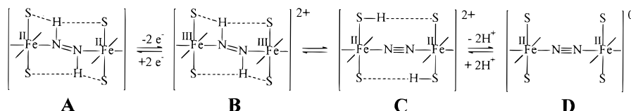
FIGURE 9. Model for the turnover states of the FeMo, FeV, or FeFe cofactors of nitrogenases stressing two unique six-coordinate Fe centers with suitable coordination spheres as binding sites for N_2 and its reduction products.
